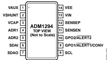
Figure 7. ADM1294 TSSOP Pin Configuration
